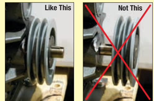
Proper Sheave Installation
