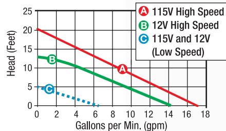
Drum Pump Kit with Polypropylene Tube and 12 VDC Motor (45827)
