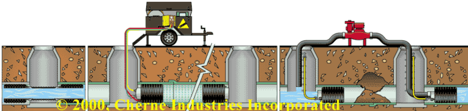
Gravity By-Pass
